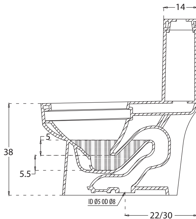
SECTIONAL VIEW
