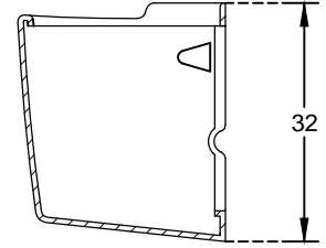
SECTIONAL VIEW
