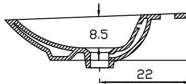
SECTIONAL VIEW
