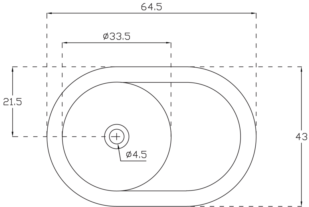
Plan View
