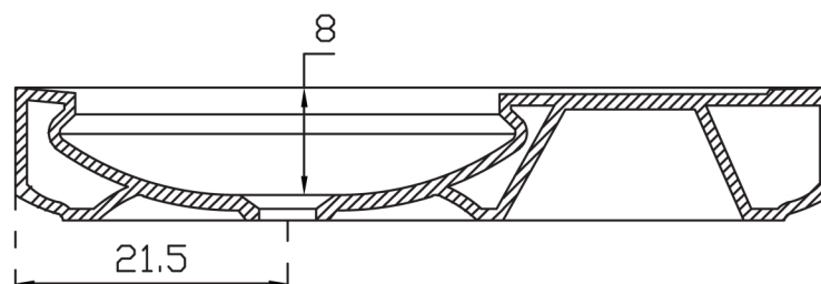
Sectional View
