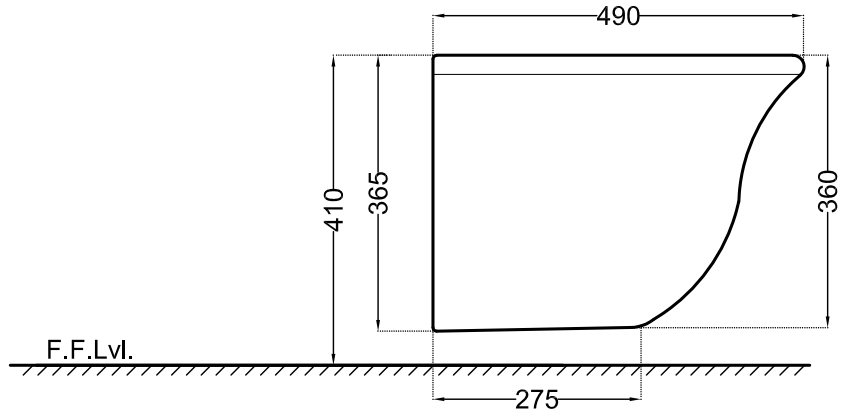
SIDE VIEW
