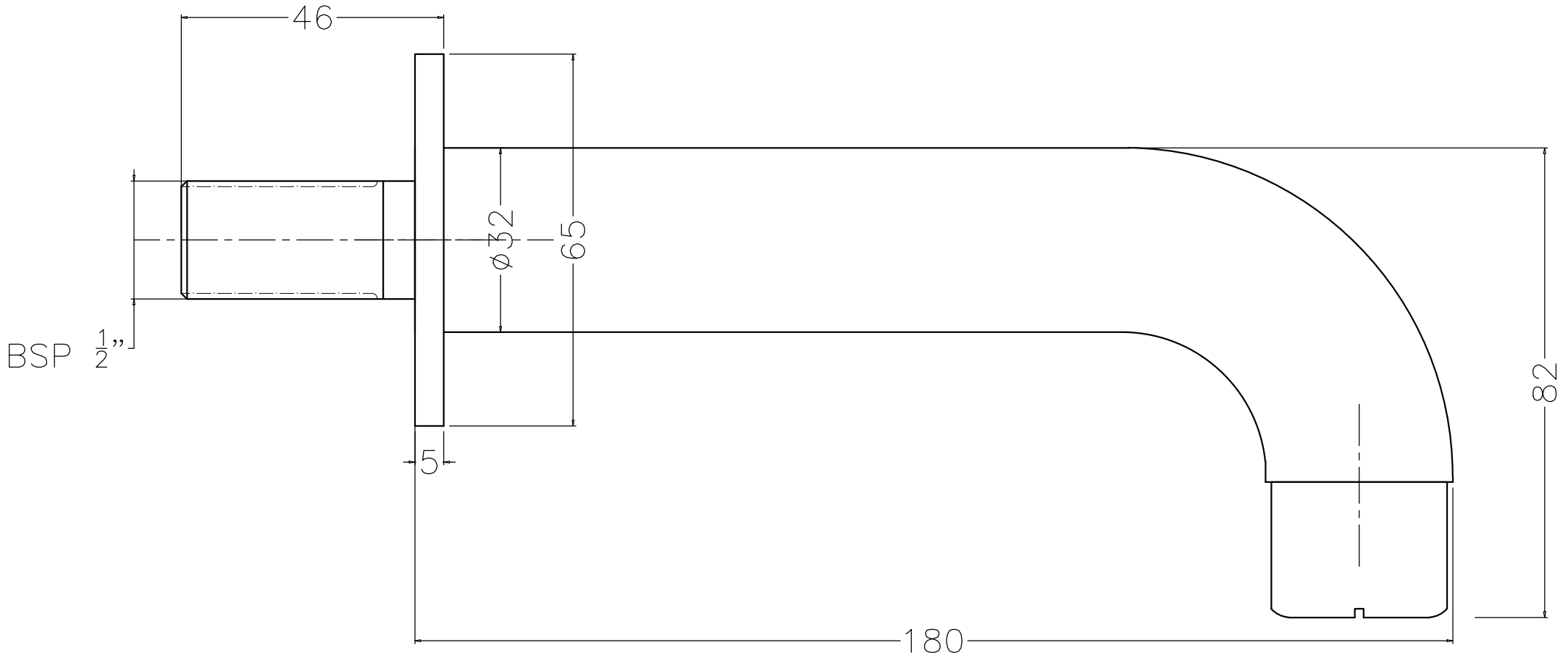
FLORA - F280007CP BATH SPOUT
