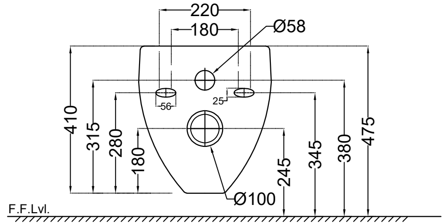
BACK VIEW
