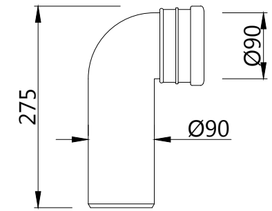
WASTE BEND
