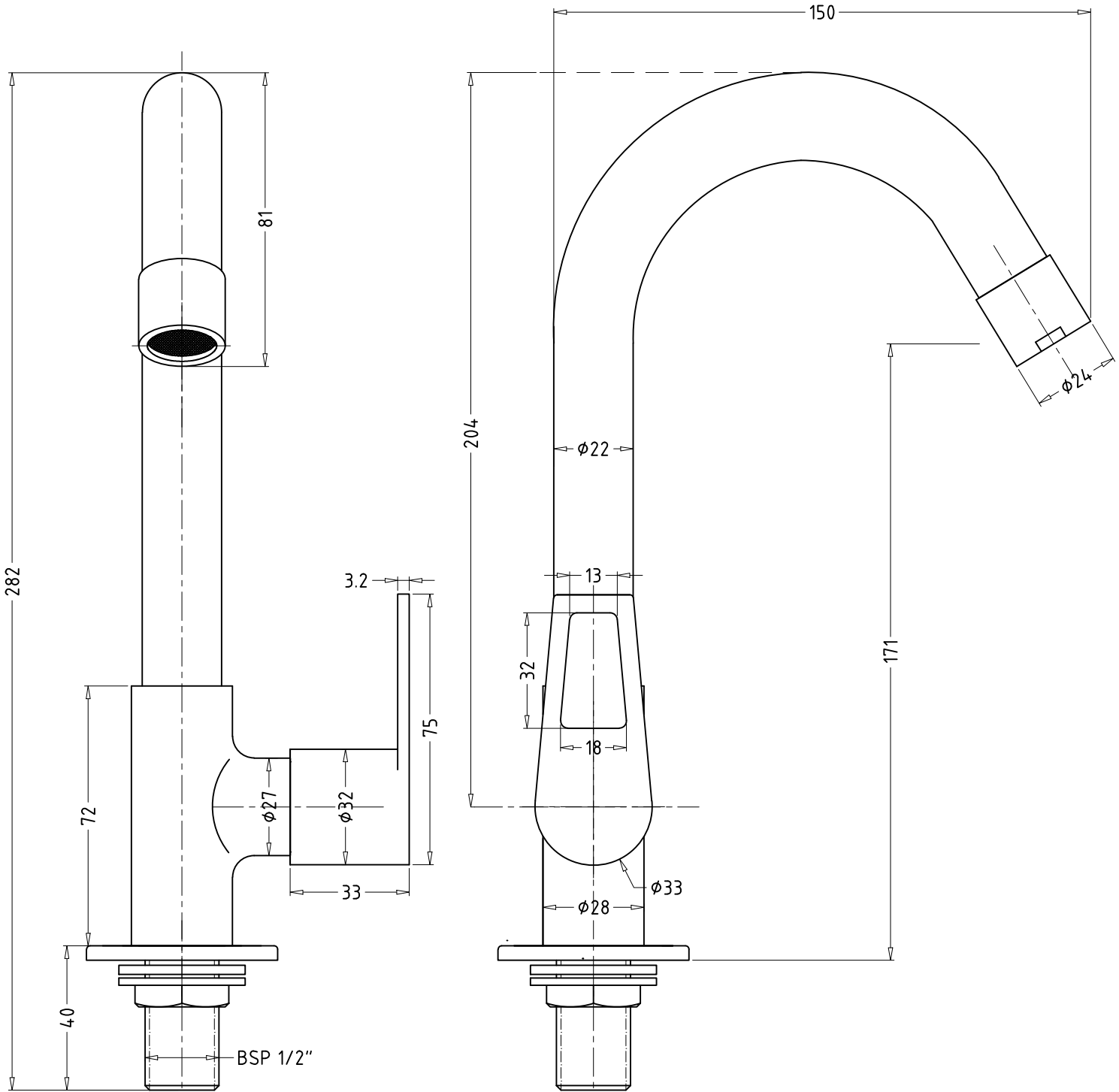
ASPIRO: F570024 SINK COCK SWIVEL SPOUT TABLE MOUNT
